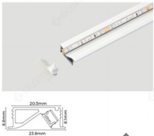
D6140-24V-4mm
