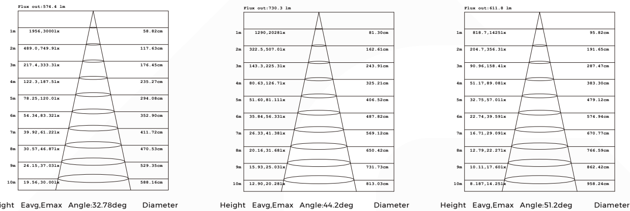
Luminous intensity distribution diagram
