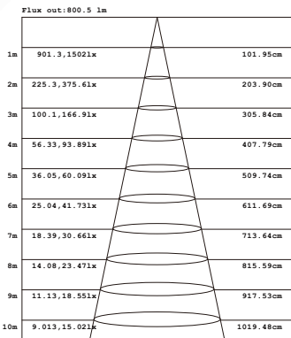
Height Eavg,Emax Angle:54.02deg Diameter
