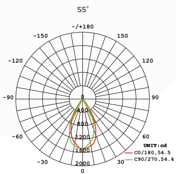
AVERAGE BEAM ANGLE(50%):54.4 DEG
