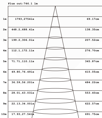
Height Eavg,Emax Angle:38.16deg Diameter
