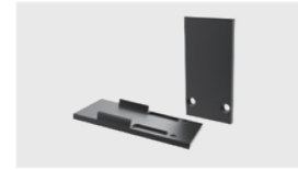
Model: EC-MH20 Material: Aluminum Size: L52*W27.2*H5.5mm Applicable model: TLS-MH2X0
