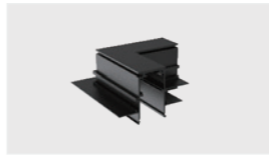
L-shaped (Downward) Model: L90-MR20(A) Material: AL6063-T5 Size: L95*W95*H46.5mm Applicable model: TLS-MR2X0(A)
