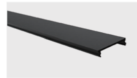
Track bind cover Model: CV-M20FB Material: PVC Size: L1000*W25.7*H5.6mm Applicable model: All straight track
