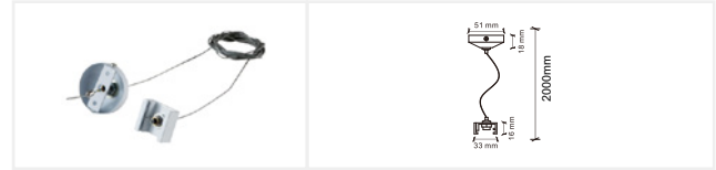
Pendant rod accessory Model: ECO-EZ0648 Size: 2000mm Colors: White/Black Applicable track: Six-wire track ECO-06X0
