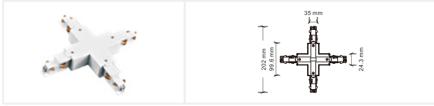
"X" shape power connector Model: ECO-0637 Size: 202*202*32mm Colors: White/Black Applicable track: Six-wire track ECO-06X0
