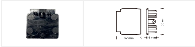
End cap Model: ECO-0632 Size: 36*32*16mm Colors: White/Black Applicable track: Six-wire track ECO-06X0
