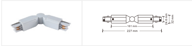
Turnable power connector
