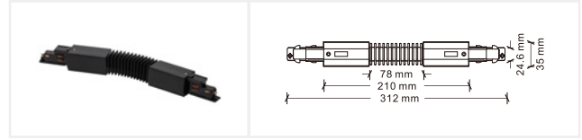
Soft power connector Model: ECO-0639 Size: 274*32.5*32mm Colors: White/Black Applicable track: Six-wire track ECO-06X0
