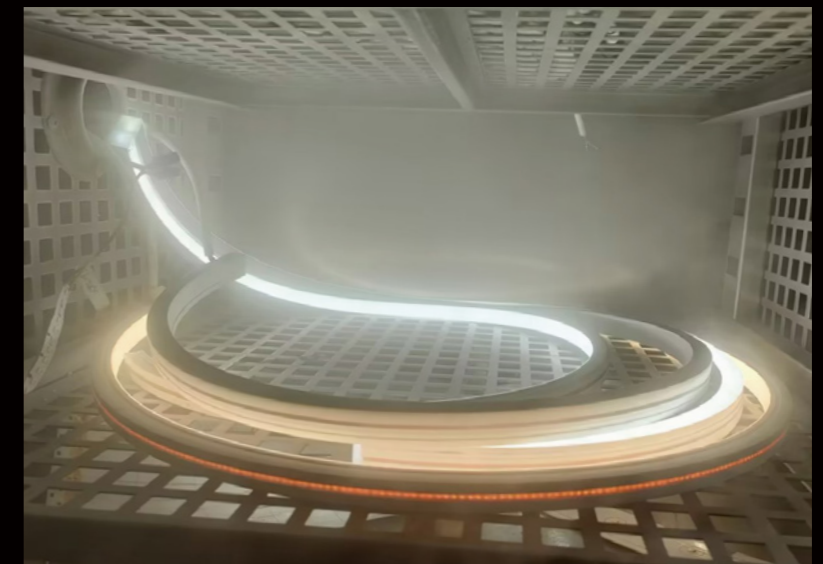
Thermal Shock Testing : -40--+100°C 1500times
