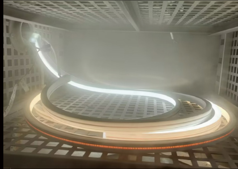
Thermal Shock Testing : -40~+110°C 1500times
