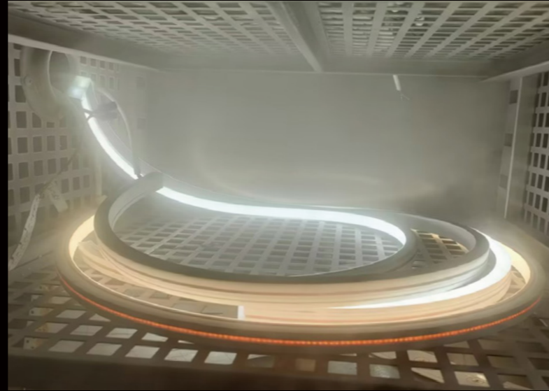
Thermal Shock Testing : -40~+100°C 1500times
